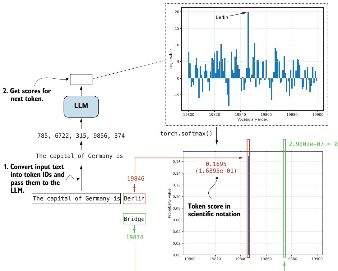
Figure 5.10 Next-token scoring. The input text is converted into token IDs and fed to the LLM, which outputs logits for the next token. After applying a softmax, these logits become probabilities, where tokens like "Berlin" receive a high probability and unlikely alternatives such as "Bridge" receive values near zero.
