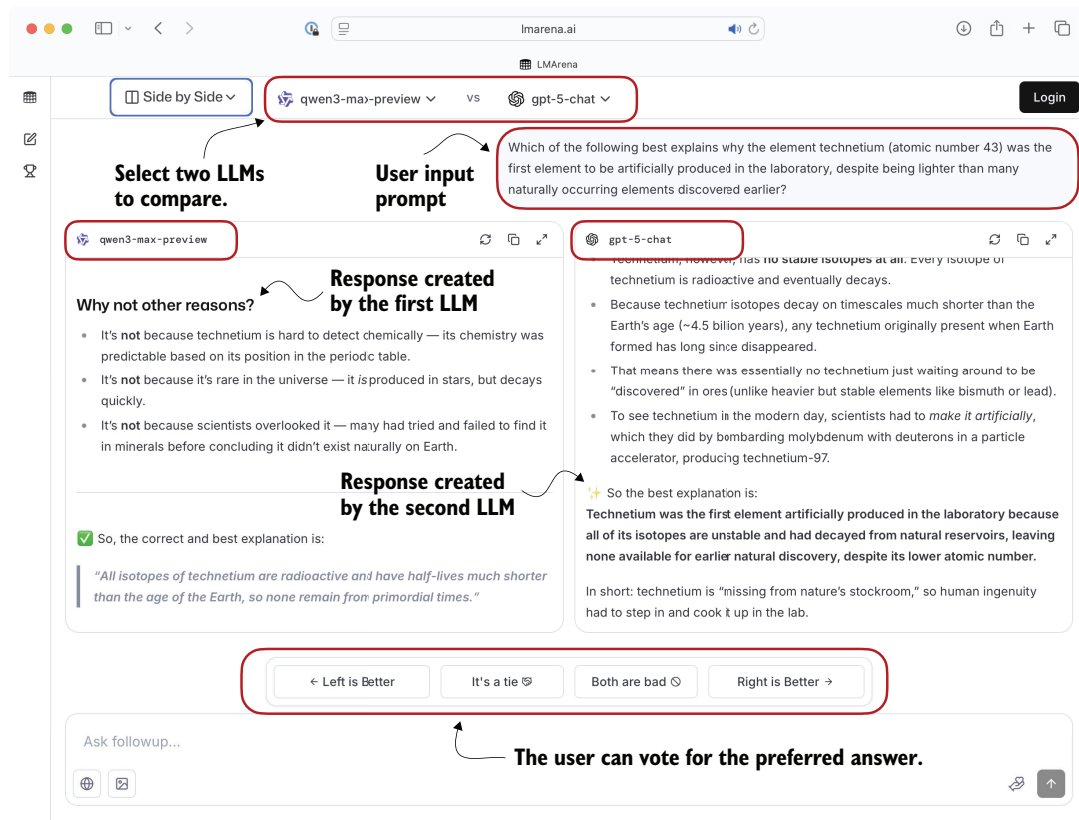
Figure F.5 Example of a judgment-based leaderboard interface (Arena). Two LLMs are given the same prompt, their responses are shown side by side, and users vote for their preferred answer.
