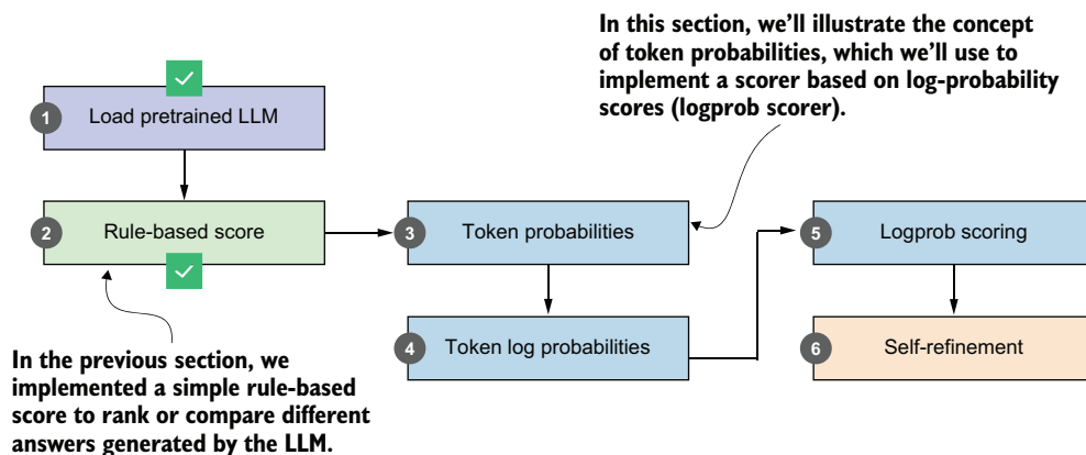
Figure 5.7 In this section, we'll move from a simple rule-based scorer to token-level probabilities. These probabilities will form the basis for the logprob scoring method that we'll use later in the self-refinement approach.
