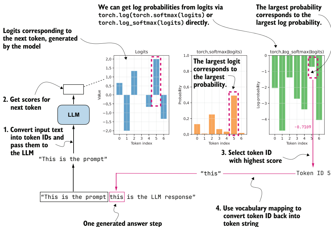
Figure 7.7 Log probability (logprob) computation of a single token ("this") in the LLM's generated answer. The LLM returns the logits of the token, which are then converted to softmax probability values via torch.softmax() or logprob values via torch.log_softmax() .
