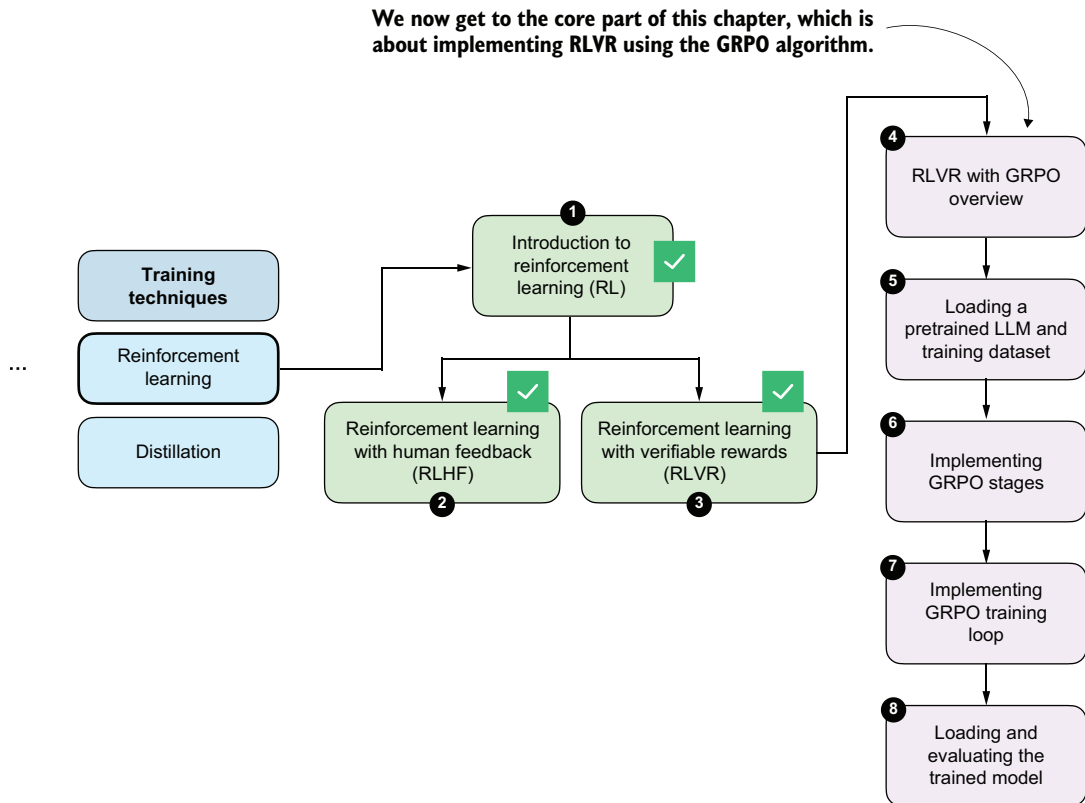
Figure 6.7 We’ve seen the two main RL approaches for LLMs, RLHF and RLVR. The remaining sections of this chapter focus on implementing RLVR using the GRPO algorithm, from loading the dataset to implementing the full training loop.
