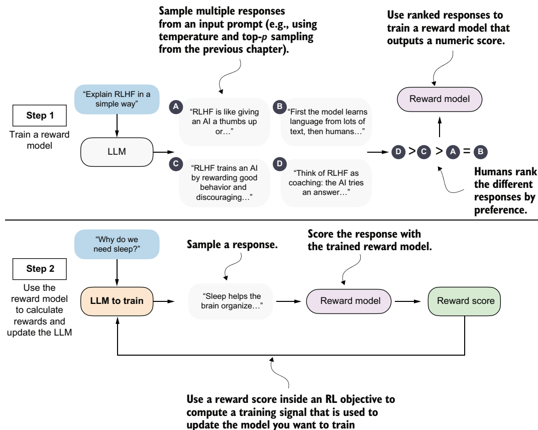
Figure 6.5 A two-stage overview of reinforcement learning with human feedback (RLHF). First, a reward model is trained on human-ranked responses to assign a preference score to each. Second, the LLM is updated using these reward scores within an RL objective to encourage preferred responses and discourage less desirable ones.
